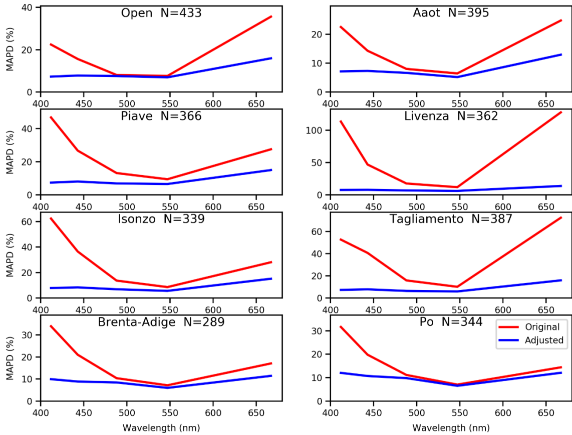
Figure 1. MAPD calculated at the virtual buoys for the original (red) and adjusted Rrs (blue) for images acquired in temporal proximity by the different VGOCS sensors.
