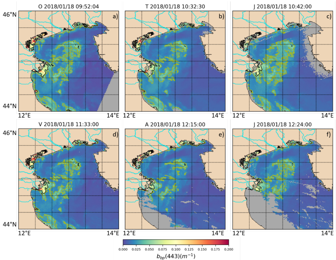
Figure 2. Analysis of the b_{bp}(443) variability during the 18 th of January 2018, derived from the adjusted VGOCS Rrs. The yellow and black isolines identify the b_{bp}(443) area of 0.03\text{m}^{-1} and 0.06\text{m}^{-1} respectively.
